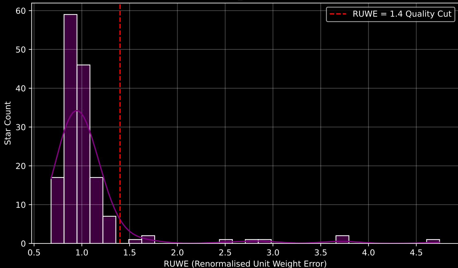
GAPOGEE DR17 Field [284-31-O_TESS] RUWE Distribution (n= 155)
