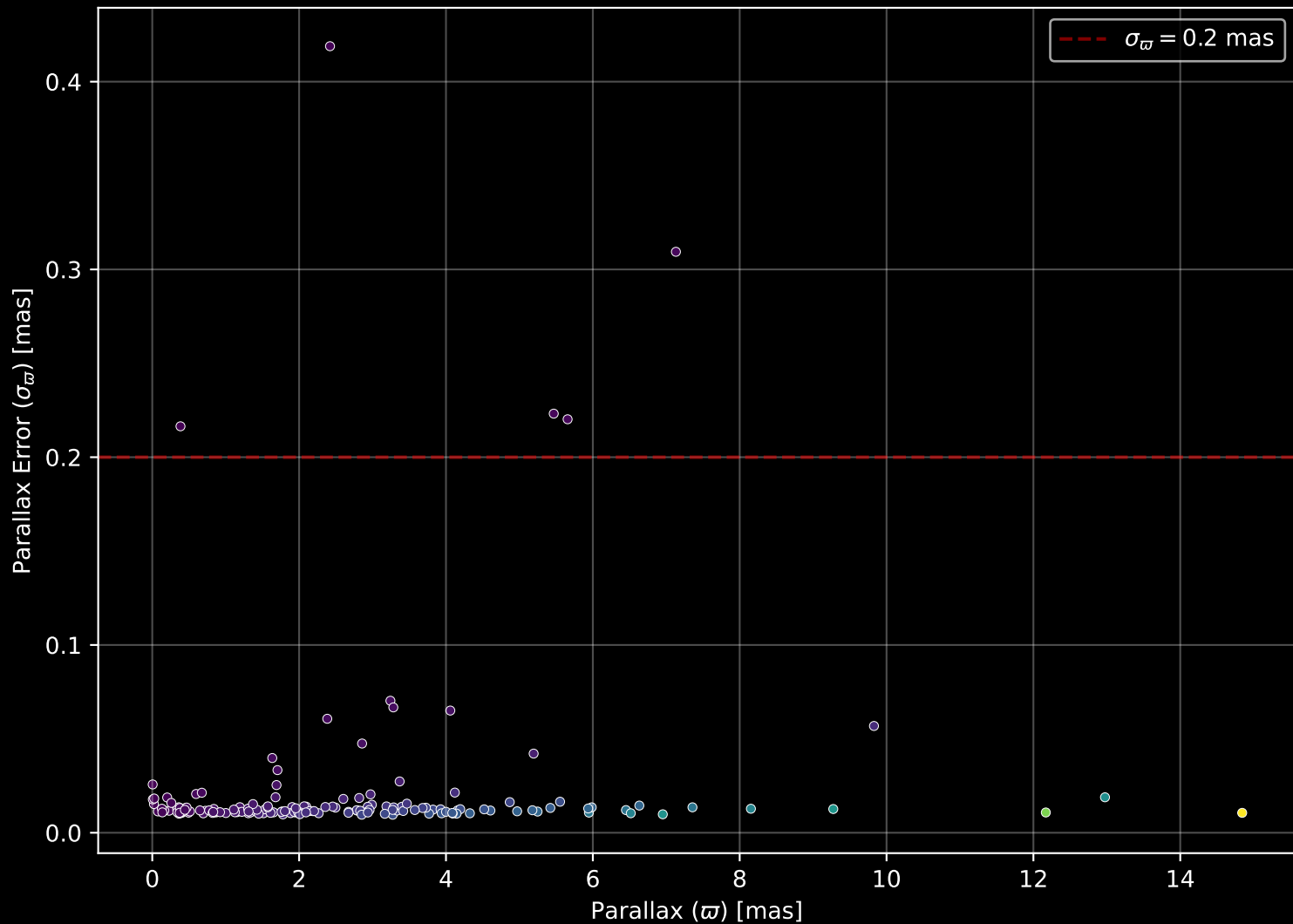
APOGEE DR17 Field: [284-31-O_TESS] Parallax Quality (n= 163)
