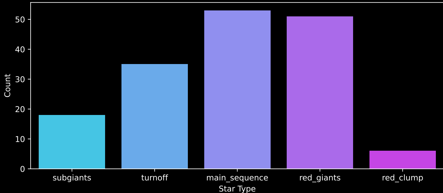
APOGEE DR17 Field: [284-31-O_TESS] Count plot of Star Type
