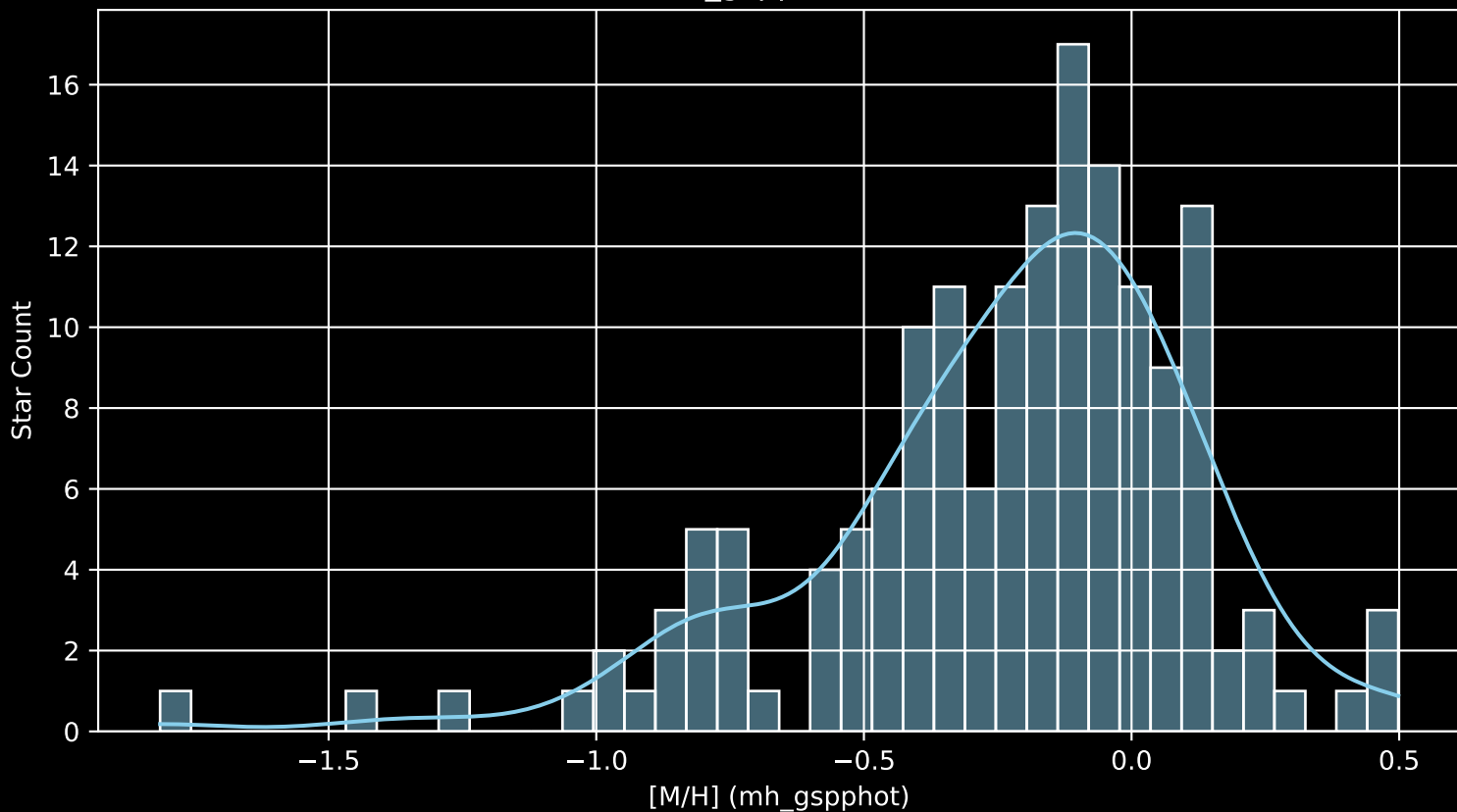
APOGEE DR17 Field: [284-31-O_TESS [M/H] (mh_gspphot) (n= 161)
