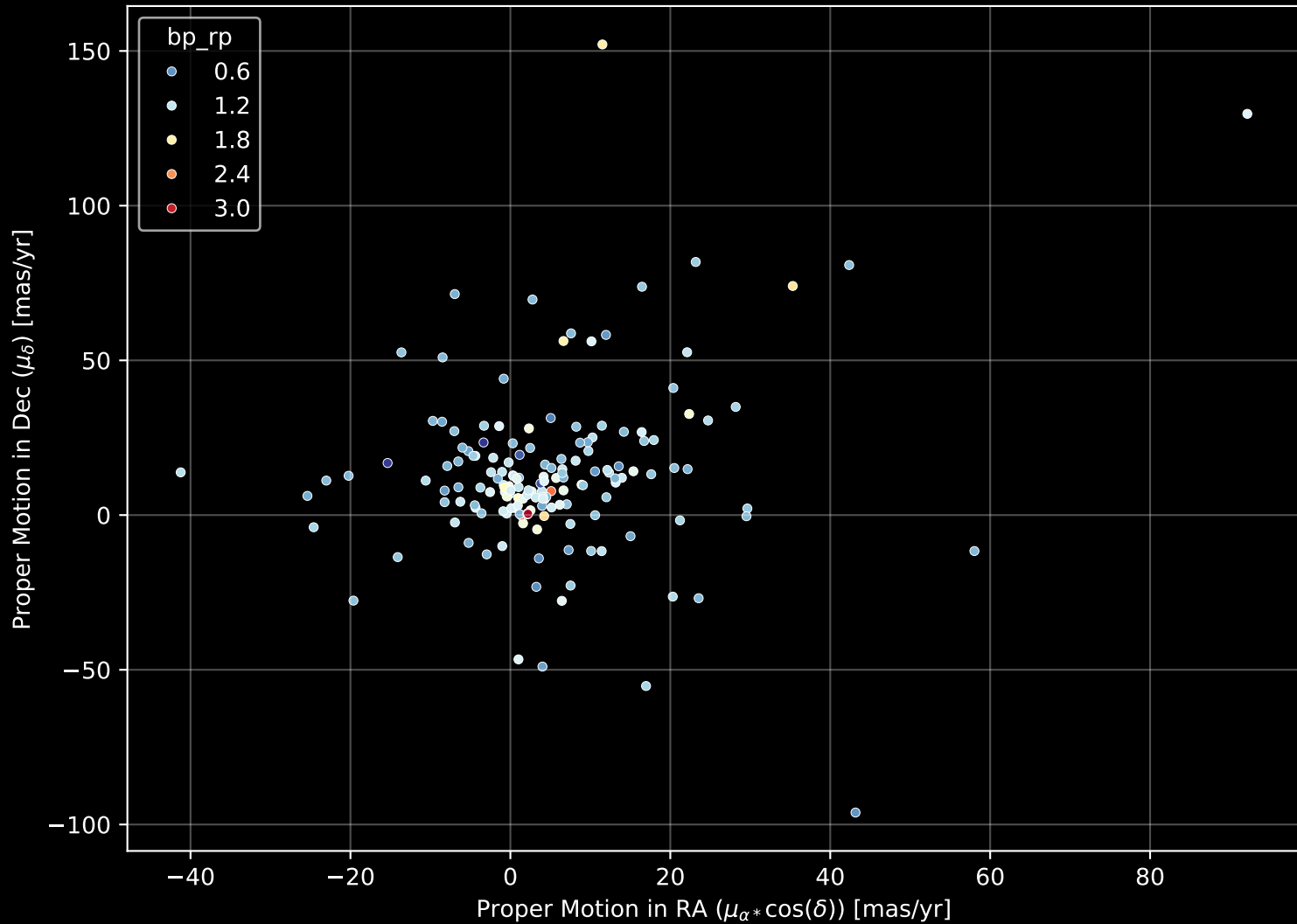
APOGEE DR17 Field: [284-31-O_TESS] Proper Motion Diagram (n= 163)
